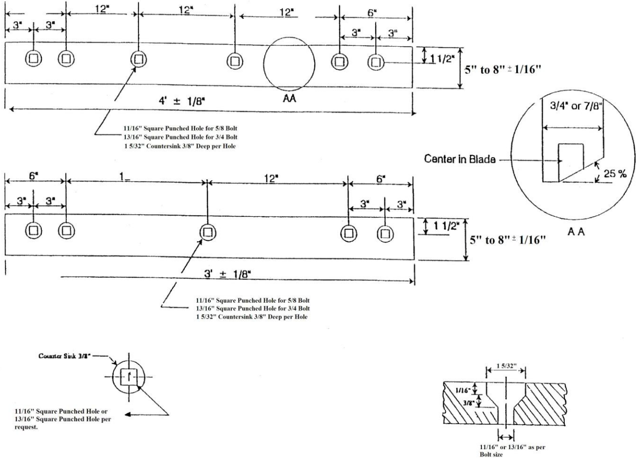
Plan of Carbide Tipped Snowplow Blades
