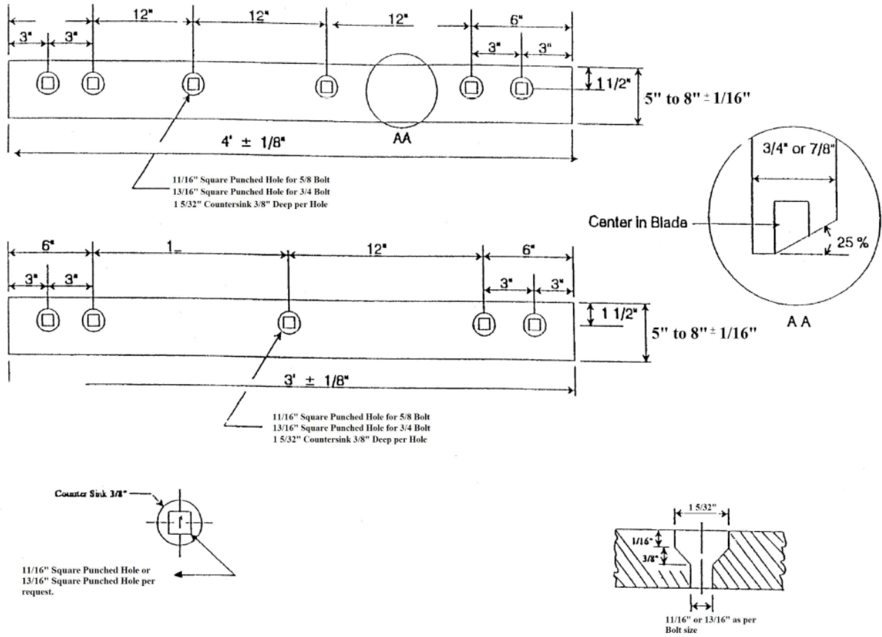
Plan of Carbide Tipped Snowplow Blades
