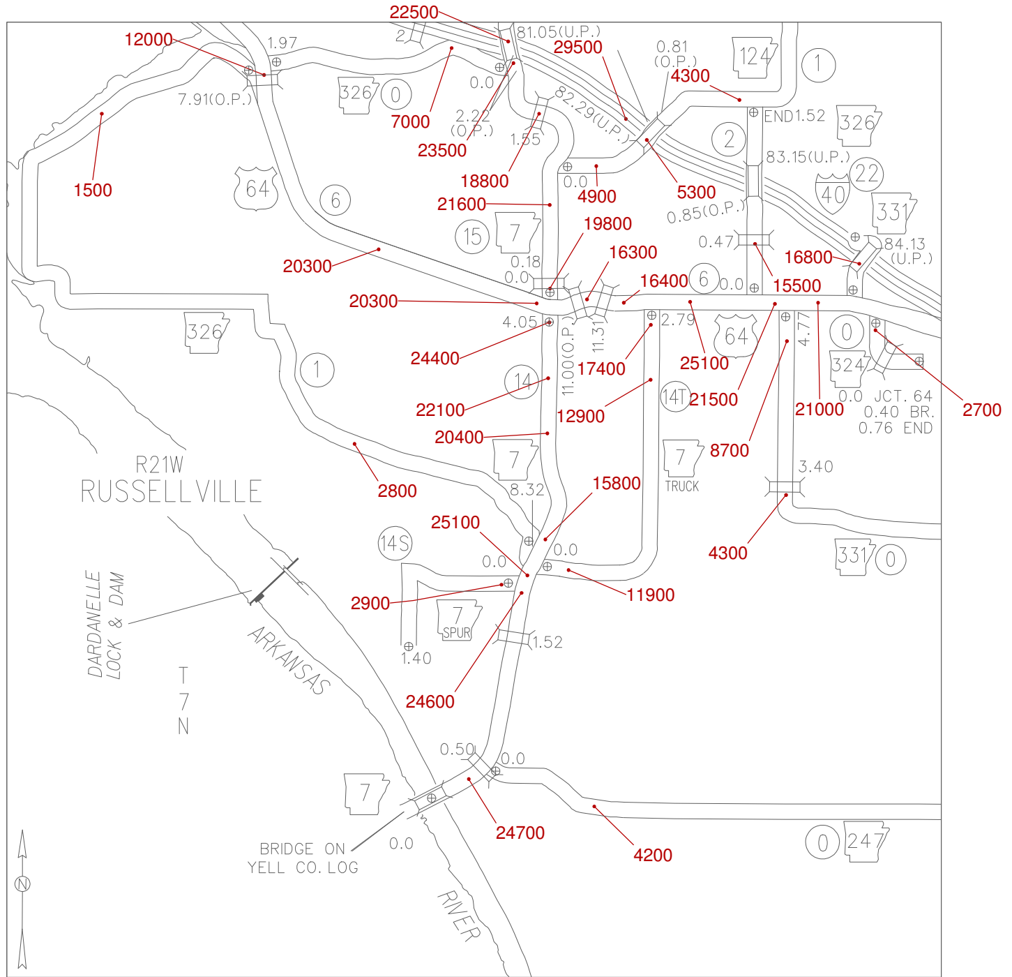
2007 ANNUAL AVERAGE DAILY TRAFFIC ESTIMATES
